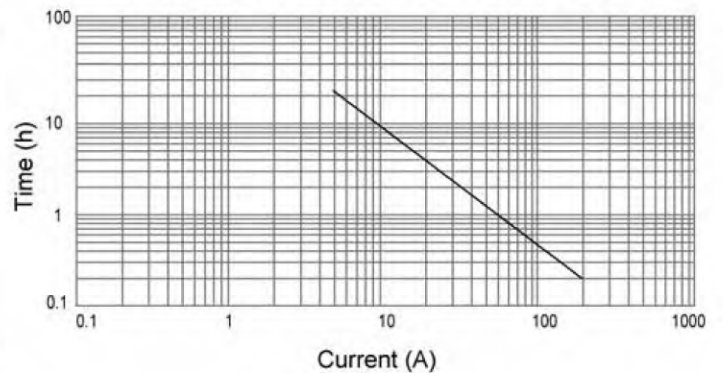
DISCHARGE CURRENT V'S TIME 25°C (77 ° F)
