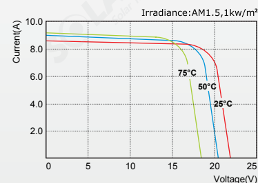
SLP150-12C1D2 I-V Curves
