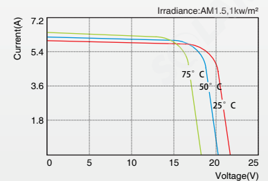
SLP100-12M I-V Curves
