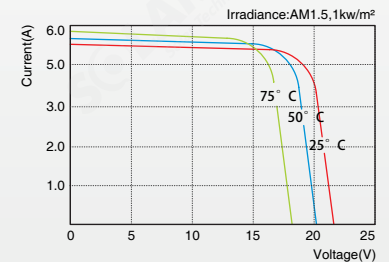
SLP090-24U I-V Curves
