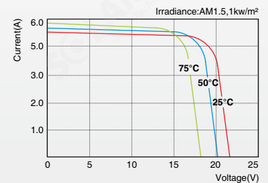
SLP085-12U I-V Curves
