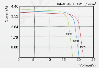
SLP060-12U I-V Curves
