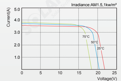
SLP060-12C1D2 I-V Curves
