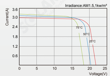
SLP050-12C I-V Curves
