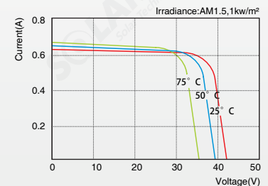
SLP020-24R I-V Curves
