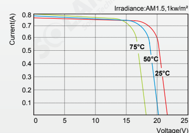
SLP012-12C1D2 I-V Curves
