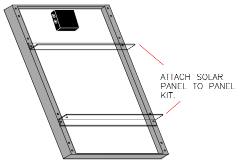
BACK VIEW OF SOLAR MODULE SHOWING HOW TO ATTACH MODULE TO PANEL KIT.
