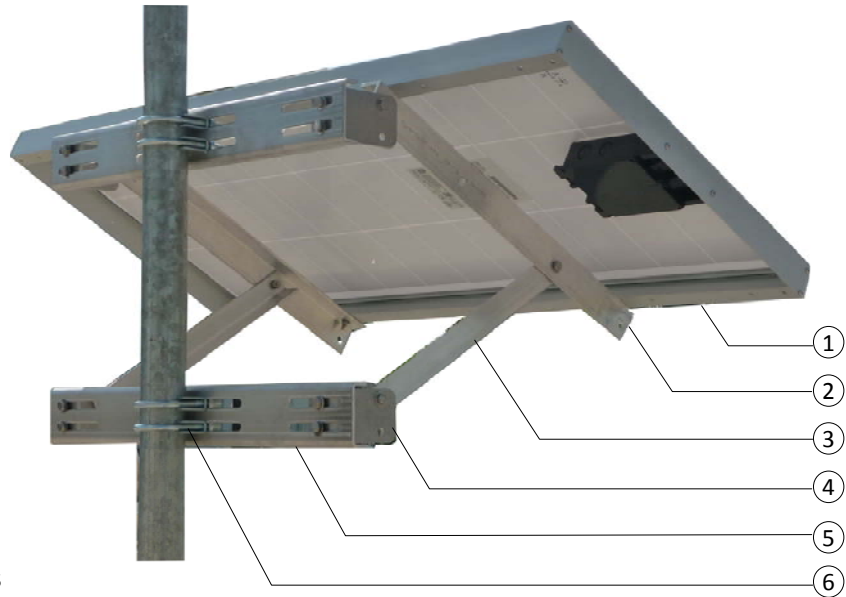
Figure 1. Mounting kit components
