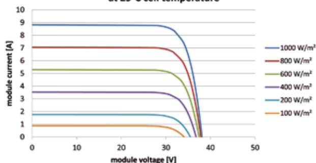
IV-curves for SolarWorld Sunmodule Plus SW 265 mono at 25°C cell temperature
