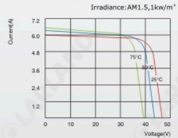
SLP200-24U I-V Curves
