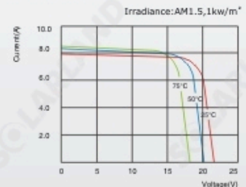
SLP130-12 I-V Curves
