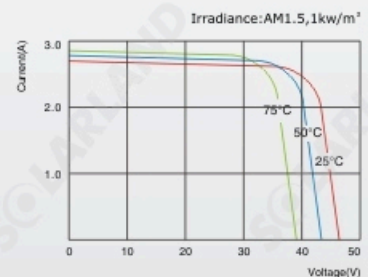
SLP085-24U I-V Curves
