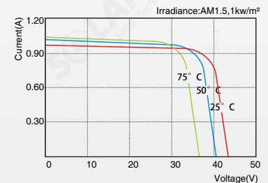
SLP030-24U I-V Curves
