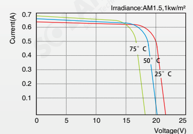
SLP010-12U I-V Curves
